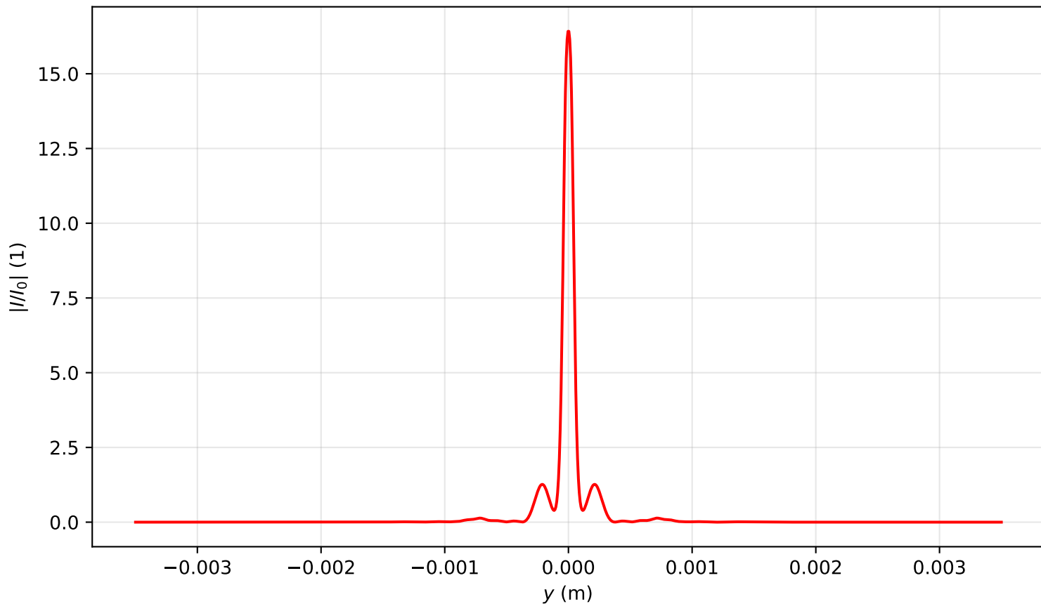
Intensity profile I(x=0, y, z=0.955)/I_0 , P_{in}=6.5P_{cr} , artificial time
